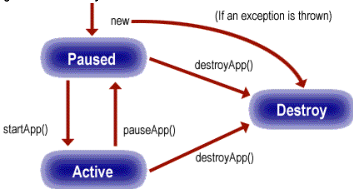
Figure 1. MIDlet life cycle
